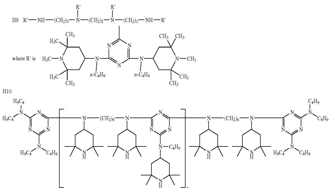
[0166] H8 bis(2,2,6,6-tetramethyl-4-piperidyl)sebacate
